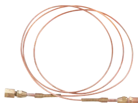
Remote connection 49-62: 6 ft copper - 300 psig max 49-62HP: 6 ft copper - 2500 psig max 49-210: 12 ft 316 SS - 3000 psig
